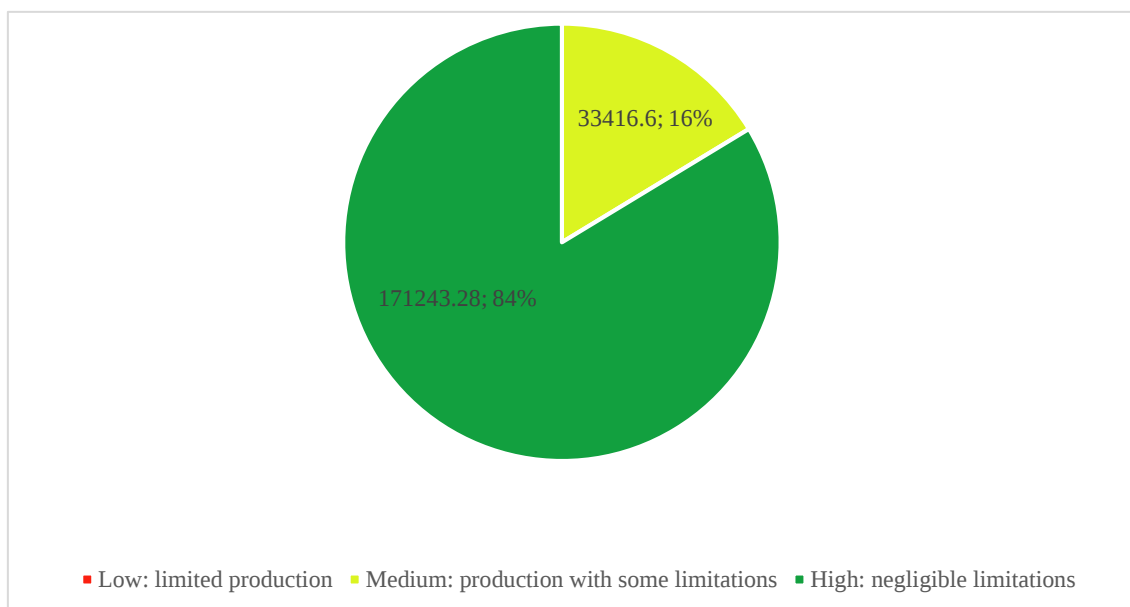
Figure 3. Distribution of land suitability classes.
